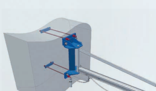
Wall mounting
